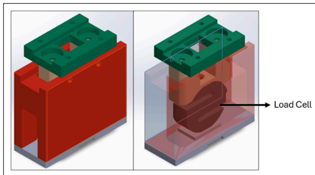
Figure 4. Load cell protective fixture.
