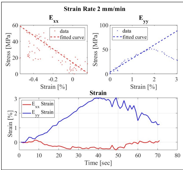
Figure 5. Strain rate 2 mm/min Ncorr results (a) E_{xx} stress-strain curve (b) E_{yy} stress-strain curve (c) Average strain for E_{xx} and E_{yy} .
