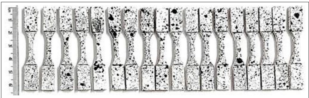
Figure 2. Surface spackle pattern preparation of tested 18 specimens.
