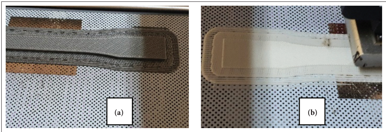
Figure 8. Printing of specimens with linear infill pattern with (a) 30 % (b) 60 % infill densit.
