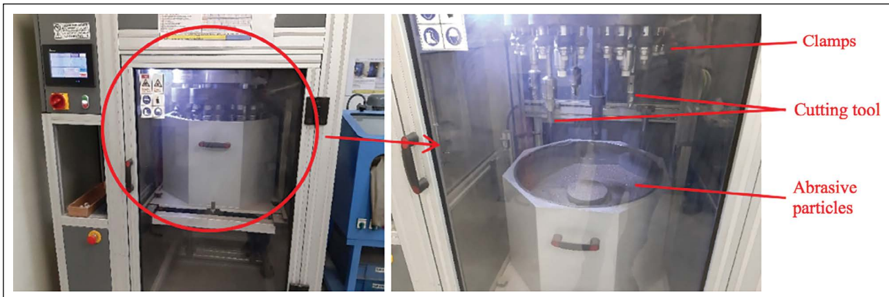
Figure 3. Drag finishing machine used in this study.
