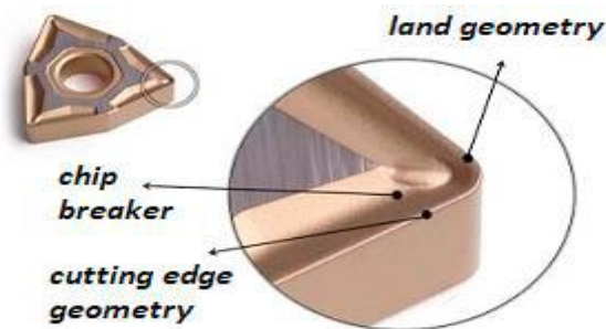
Figure 11. Geometry of cutting inserts
