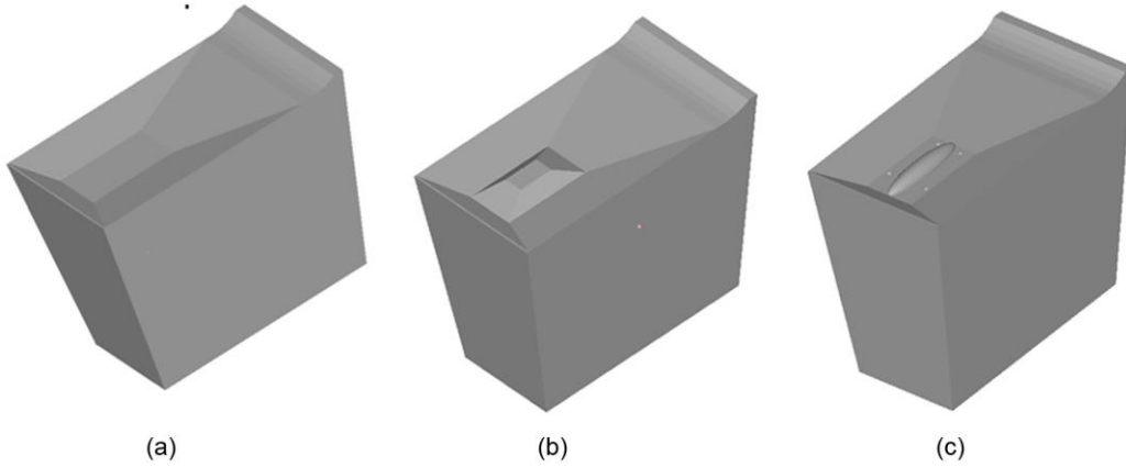
Figure 5. Simulation diagram of the different chip breakers: (a) without chip breaker (b) squared chip breaker, and (c) elliptical chip breaker.
